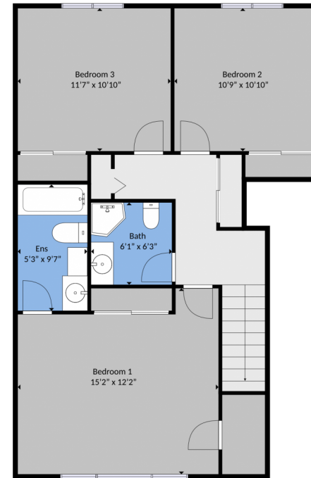
2nd Floor
