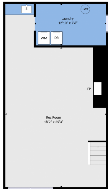
Basement
