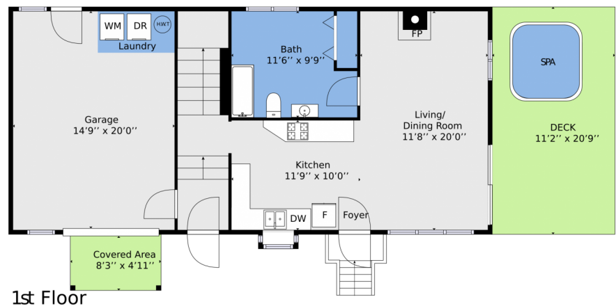
1st Floor
