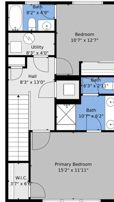
3rd Floor
