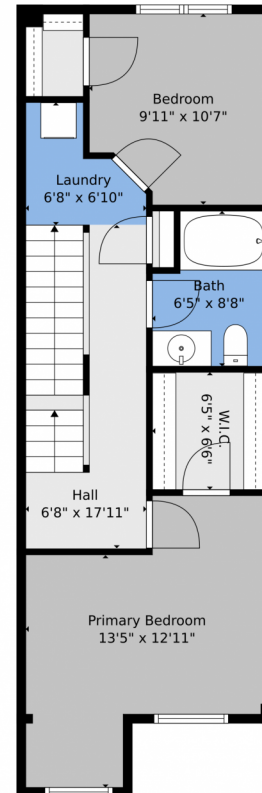
Floor 3
