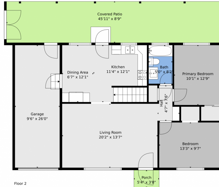
Floor 2
