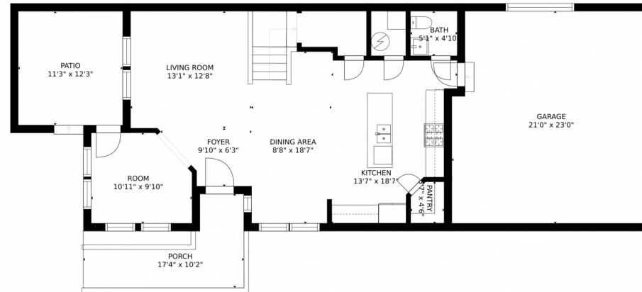
FLOOR 1
